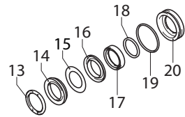
Water Seals and Piston Guides BEFORE MAY 2022
